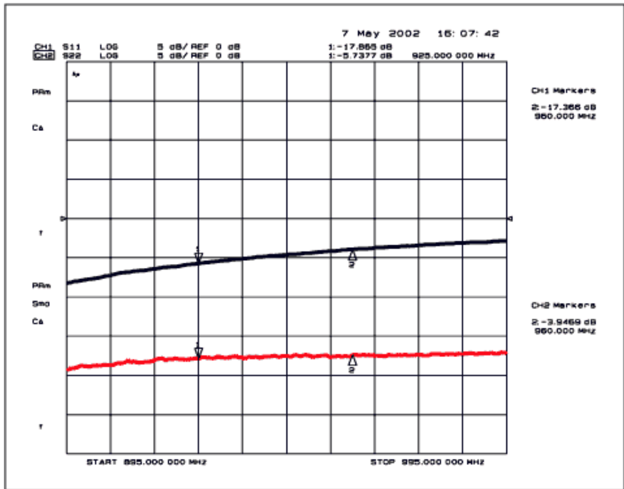
Figure 5. S11 and S22 small signal plots
